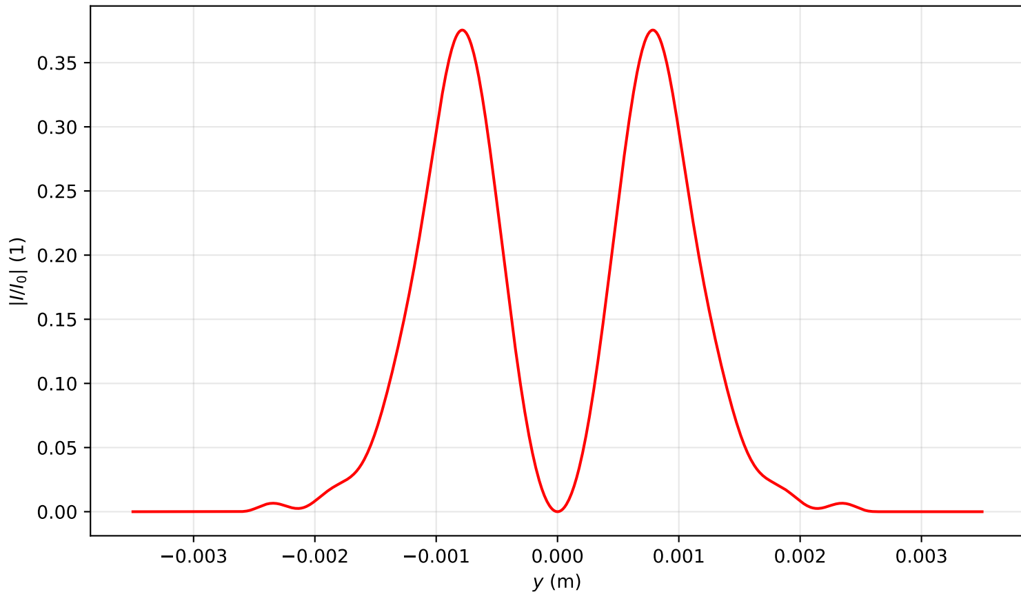
Intensity profile I(x=0, y, z=3.105)/I_0 , \text{Pin}=3.0\text{Pcr} , artificial time
